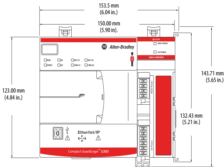
Compact GuardLogix 5380 SIL 3 Controller
